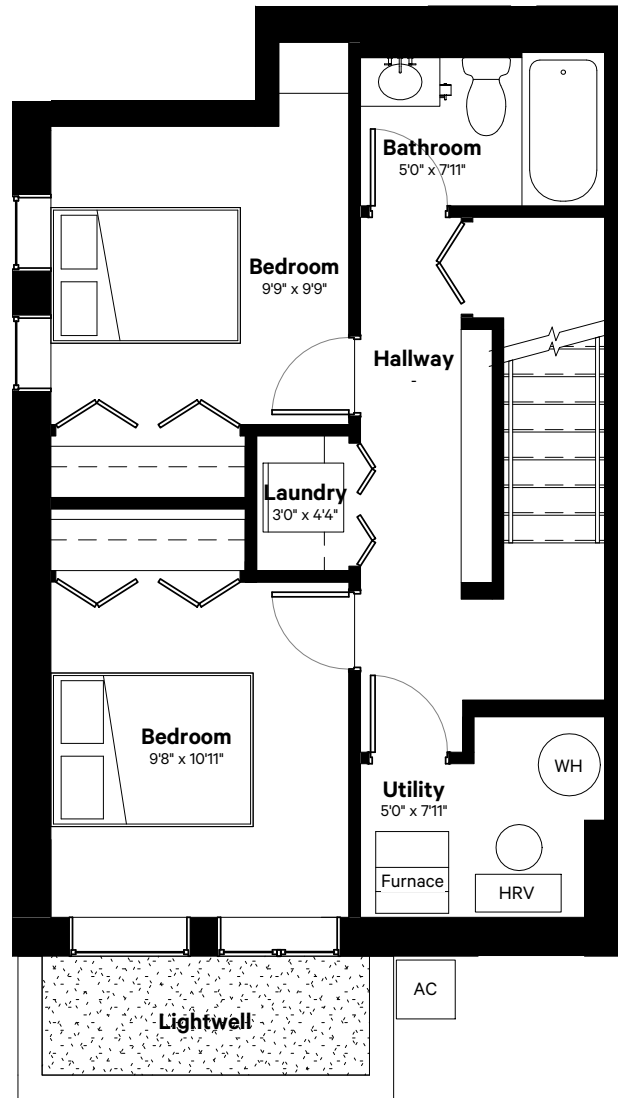
Lower Floor
