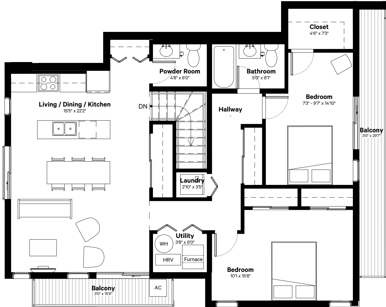
Second Floor
