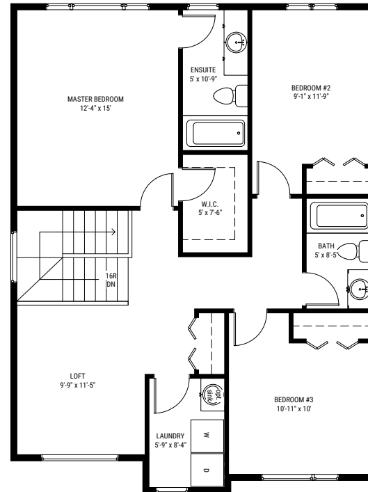
SECOND FLOOR (standard loft) 1010 sq. ft.
